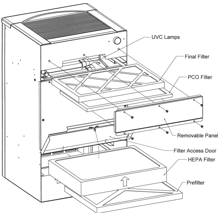
Fig. 1 – Air Cleaner Layout
