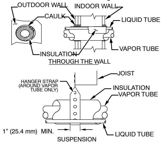
Fig. 1 - Piping Installation
